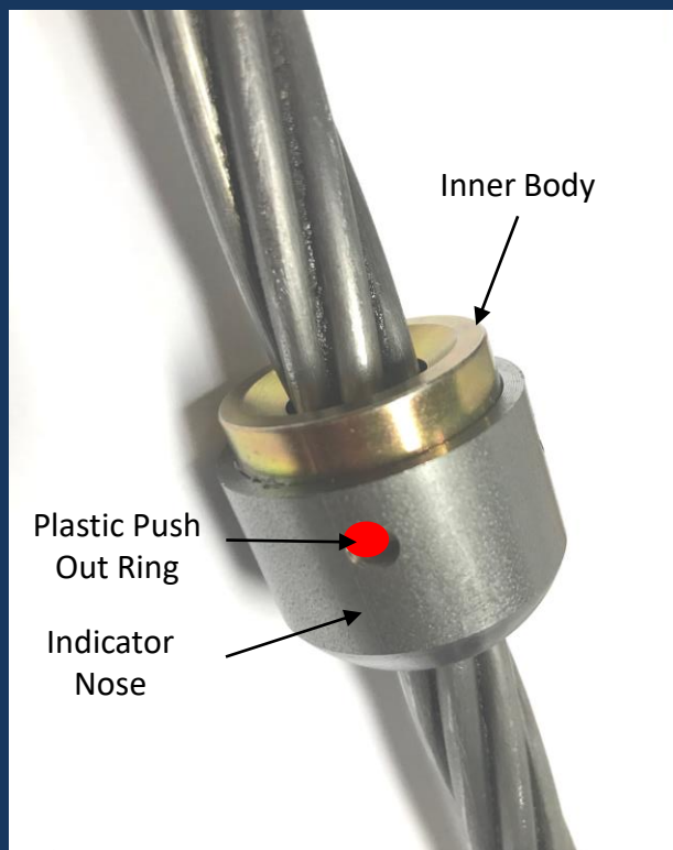
Non Activated V2 15T Event Indicator on a 15mm strand
